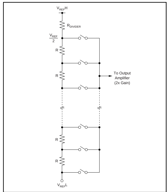
FIGURE 2. Resistor String.
