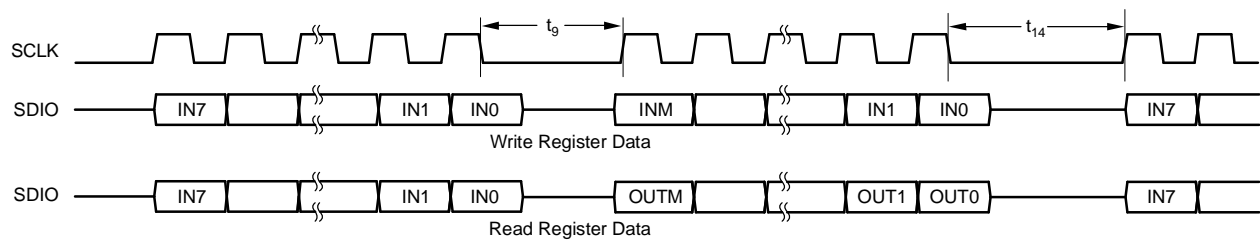
Figure 9. Serial Interface Timing ( \overline{CS} Low)
