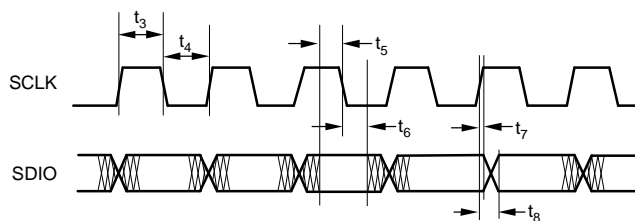
Figure 8. Serial Input/Output Timing
