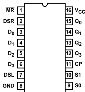
CD54HC194 (CERDIP) CD74HC194 (PDIP, SOIC, SOP, TSSOP) CD74HCT194 (PDIP, SOIC) TOP VIEW
