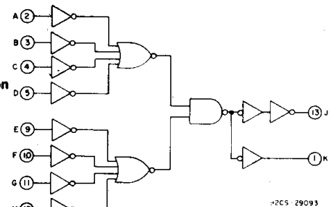
Fig. 1 – Logic diagram.
