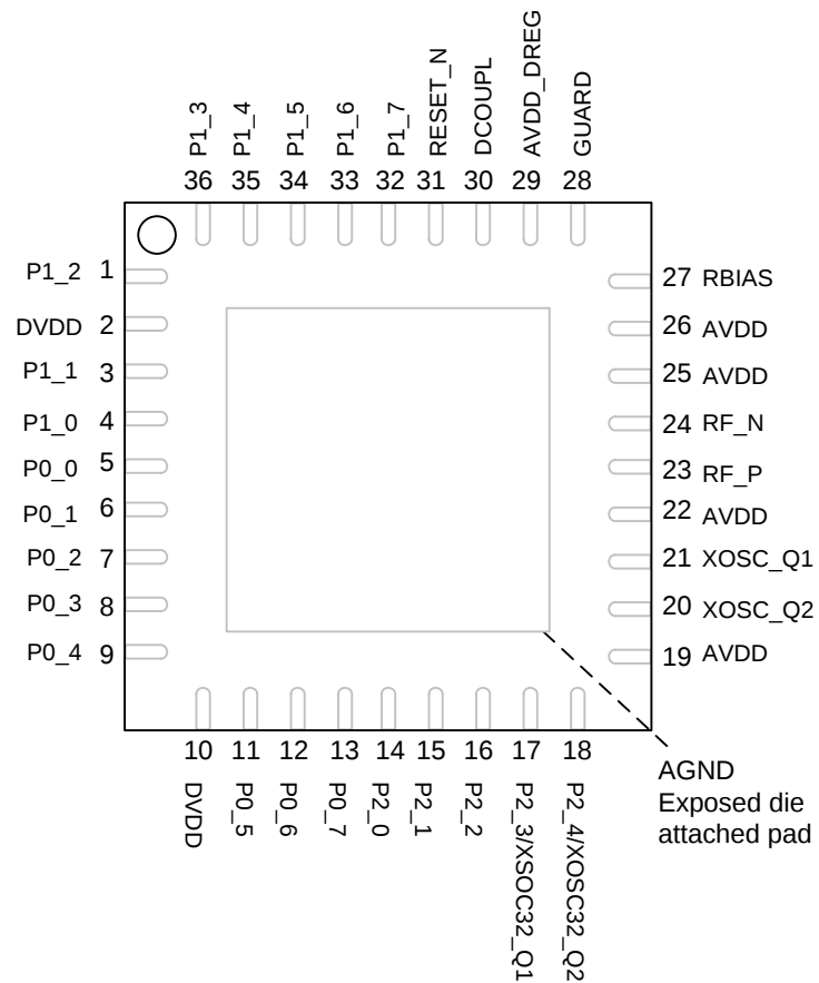
Figure 7: CC2510Fx Pinout Top View
