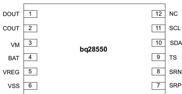
Figure 1. Top View
