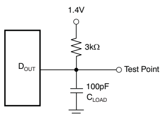
Load Circuit for t_{\text{dDO}} , t_{\text{r}} , and t_{\text{f}}
