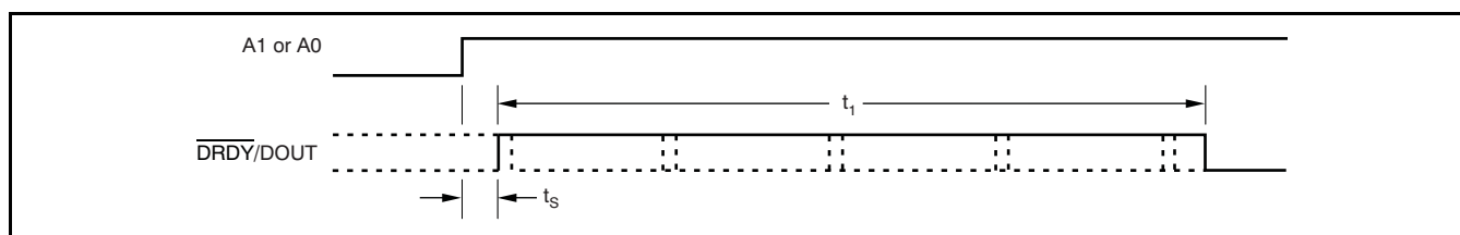
Figure 32. Example of Settling Time After Changing the Input Multiplexer
