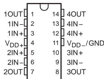
TLV2264I, TLV2264AI TLV2264Q, TLV2264AQ D, N, OR PW PACKAGE (TOP VIEW)
