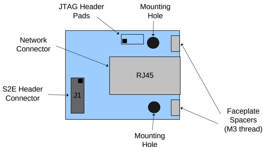
Figure 1-2. Serial-to-Ethernet Module
