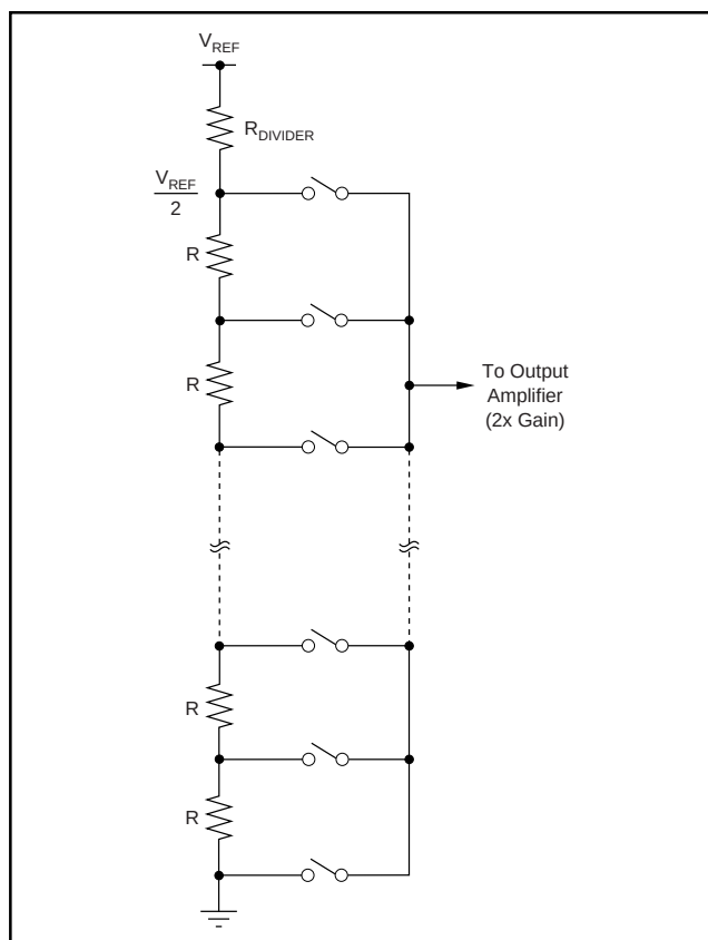
FIGURE 2. Resistor String.
