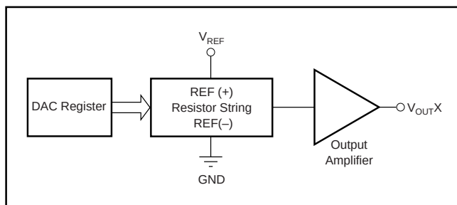
FIGURE 1. DAC8532 Architecture.
