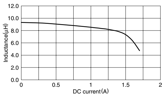
VLC5020T-100M
