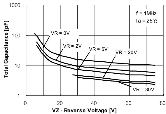
Figure 2. Total Capacitance
