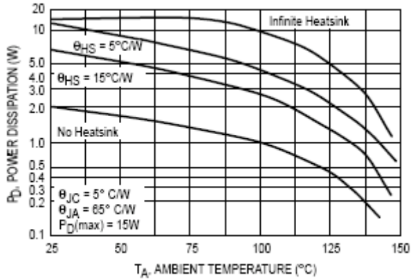
FIGURE 1 - Worst Case Power Dissipation v.s. Ambient Temperature
