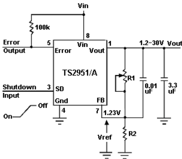
Figure 2. Adjust Voltage
