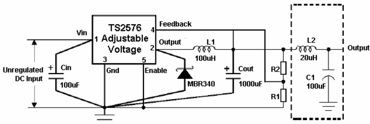
Figure 3: LC filter for Low Output Ripple
