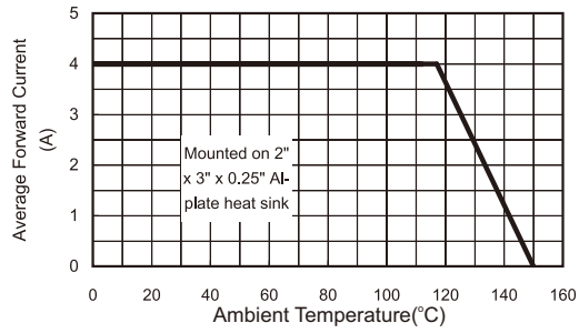
FIG 1 Maximum Derating Curve for Output Current
