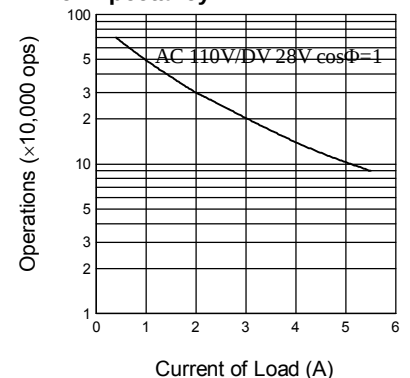
Life Expectancy
