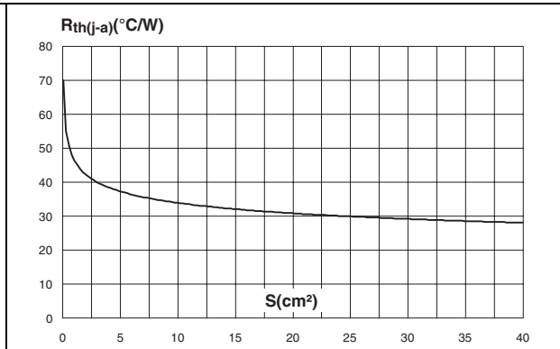
Figure 12. Thermal resistance junction to ambient versus copper surface under tab - Epoxy printed circuit board, e_{Cu} 35 \mu m (STPS20150CG only)
