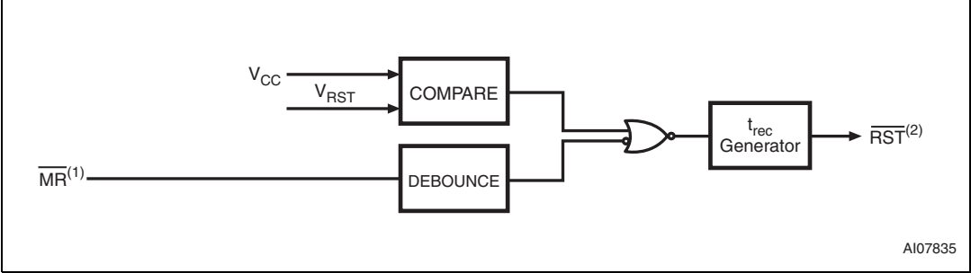
Figure 5. Block diagram
