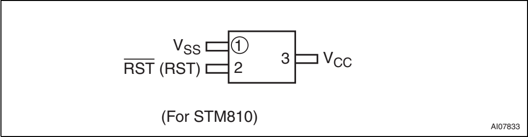
Figure 4. SOT143-4 connections
