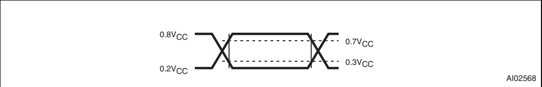
Figure 14. MR timing waveform
