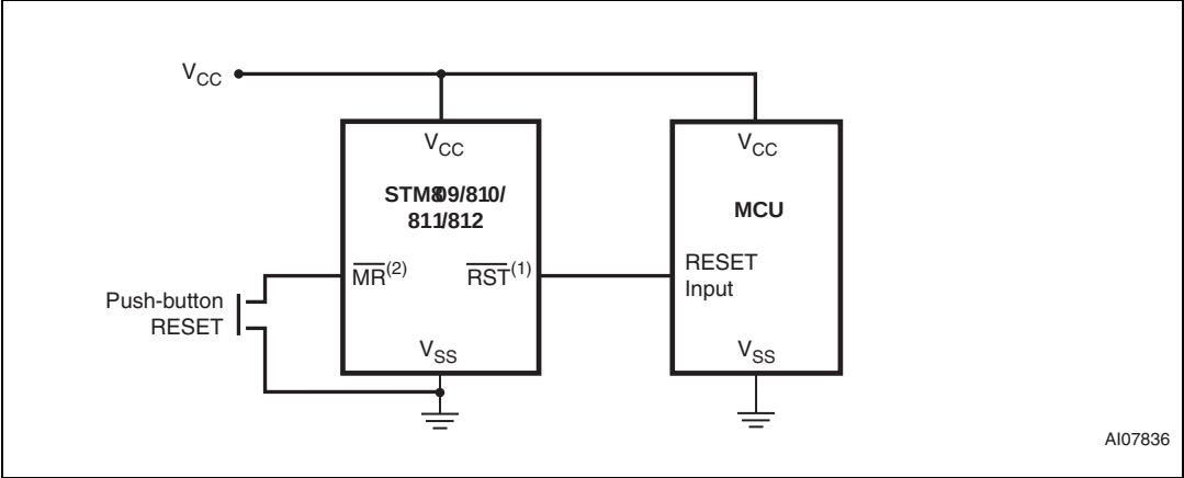
Figure 6. Hardware hookup
