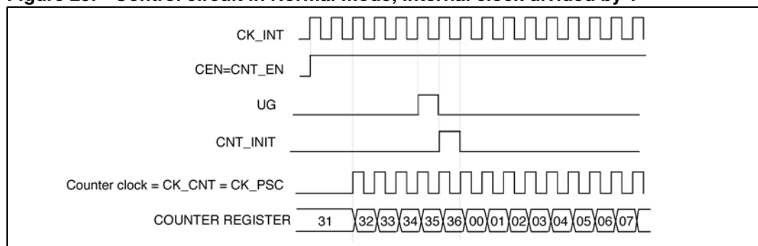
Figure 25. Control circuit in Normal mode, internal clock divided by 1
