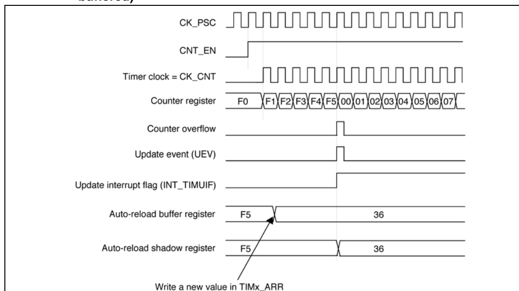
Figure 19. Counter timing diagram, update event when TIM_ARBE = 1 (TIMx_ARR buffered)
