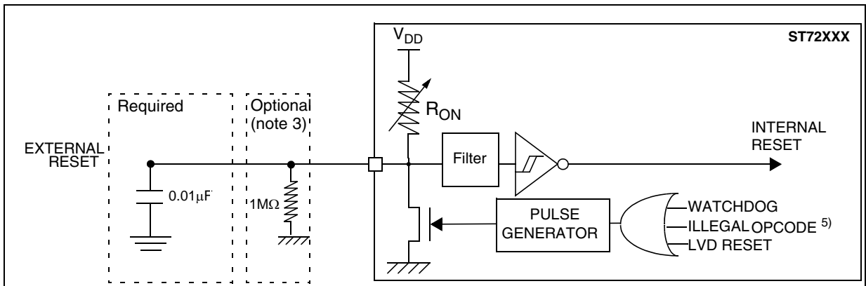
Figure 143. \overline{\text{RESET}} pin protection when LVD is disabled. 1)
