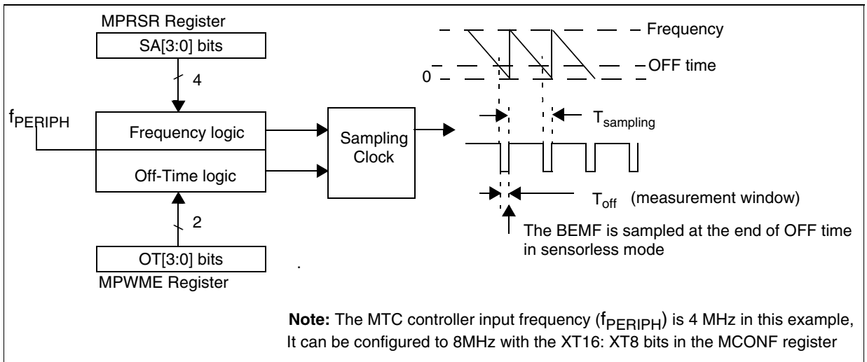
Figure 105. Sampling clock generation block
