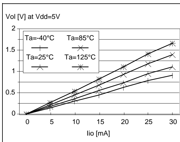
Figure 140. Typical V_{OL} at V_{DD}=5\text{V} (high-sink)
