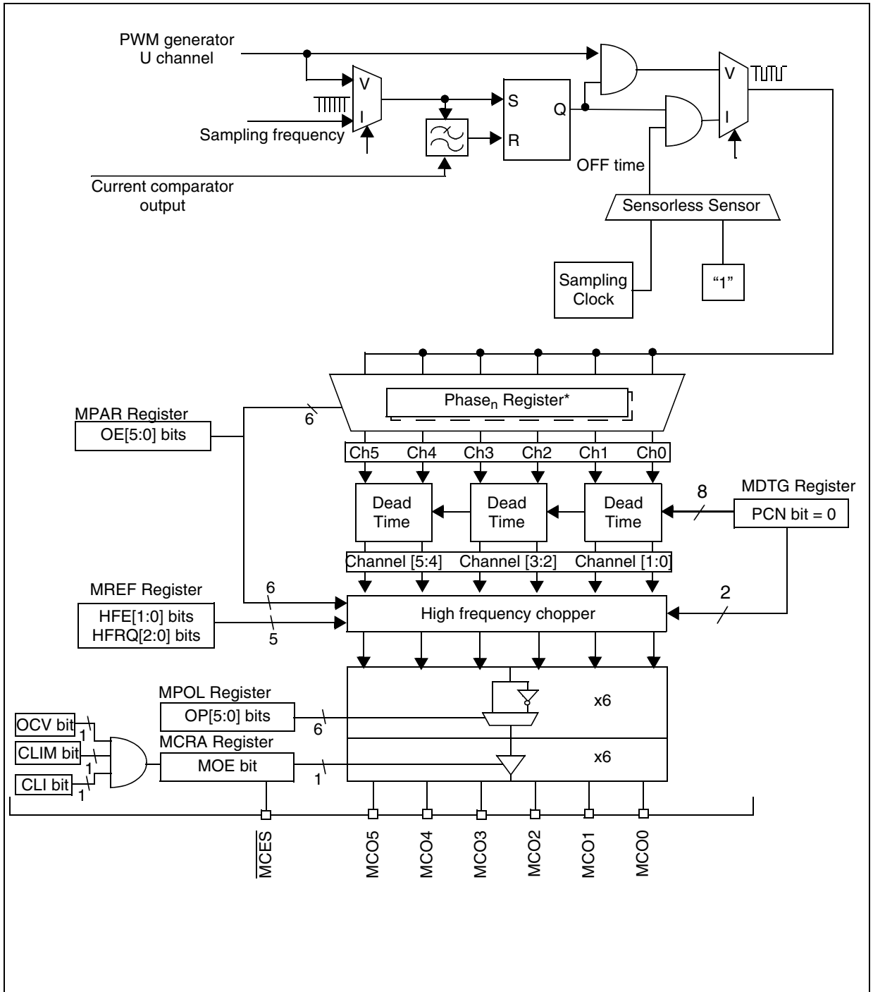
Figure 113. Channel Manager Output Block Diagram with PWM generator delivering 1 PWM signal
