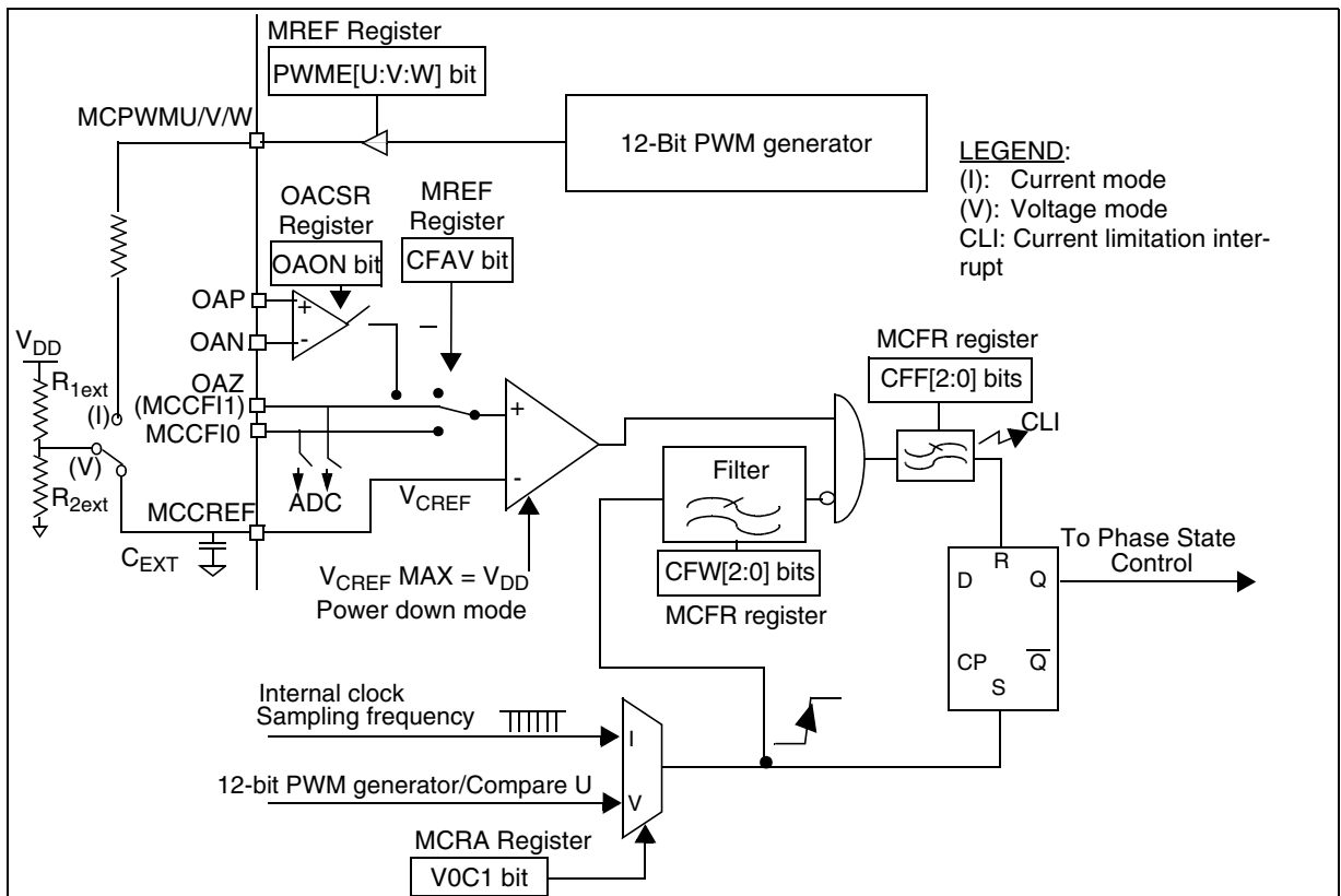
Figure 104. Current Feedback
