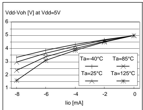
Figure 141. Typical V_{DD}-V_{OH} at V_{DD}=5\text{V}
