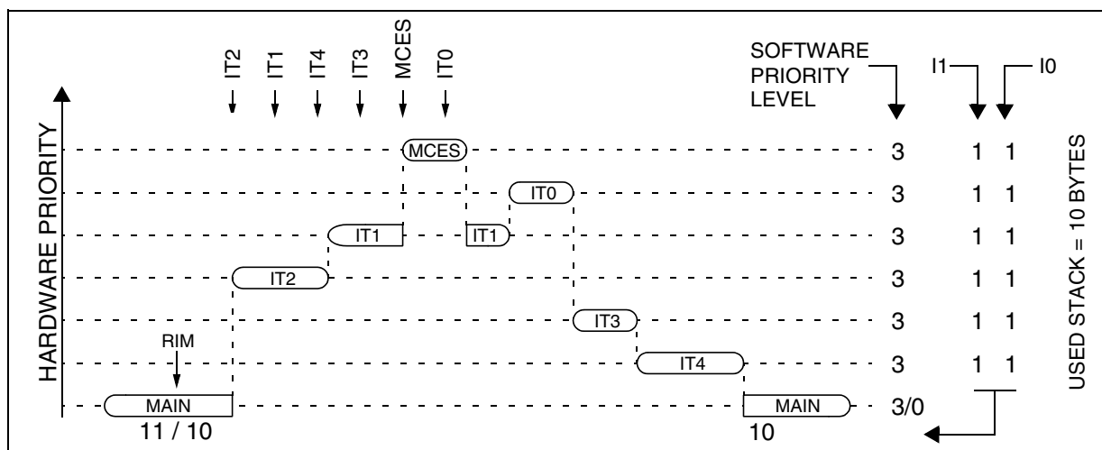
Figure 20. Concurrent Interrupt Management
