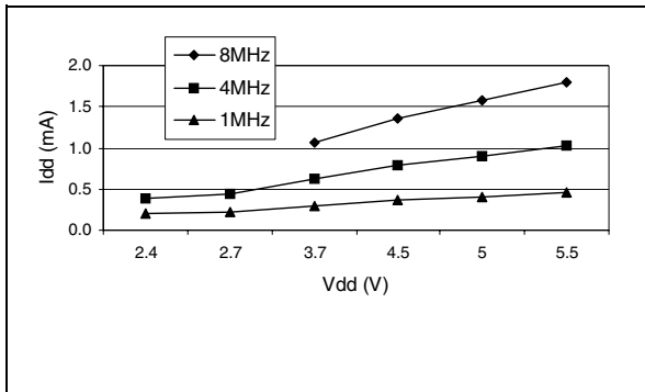
Figure 57. Typical I_{DD} in WAIT vs. f_{CPU}
