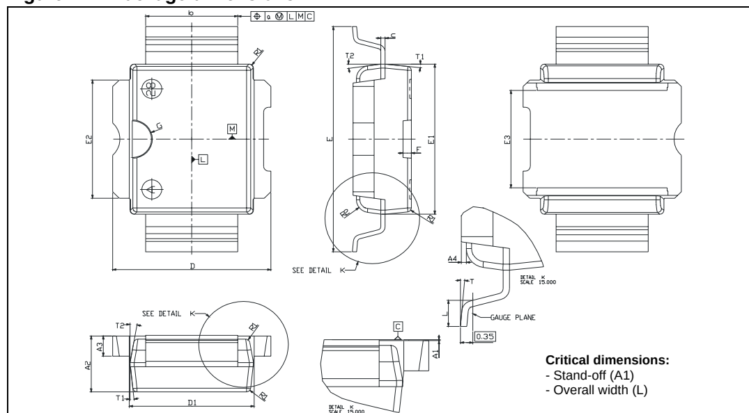
Figure 17. Package dimensions
