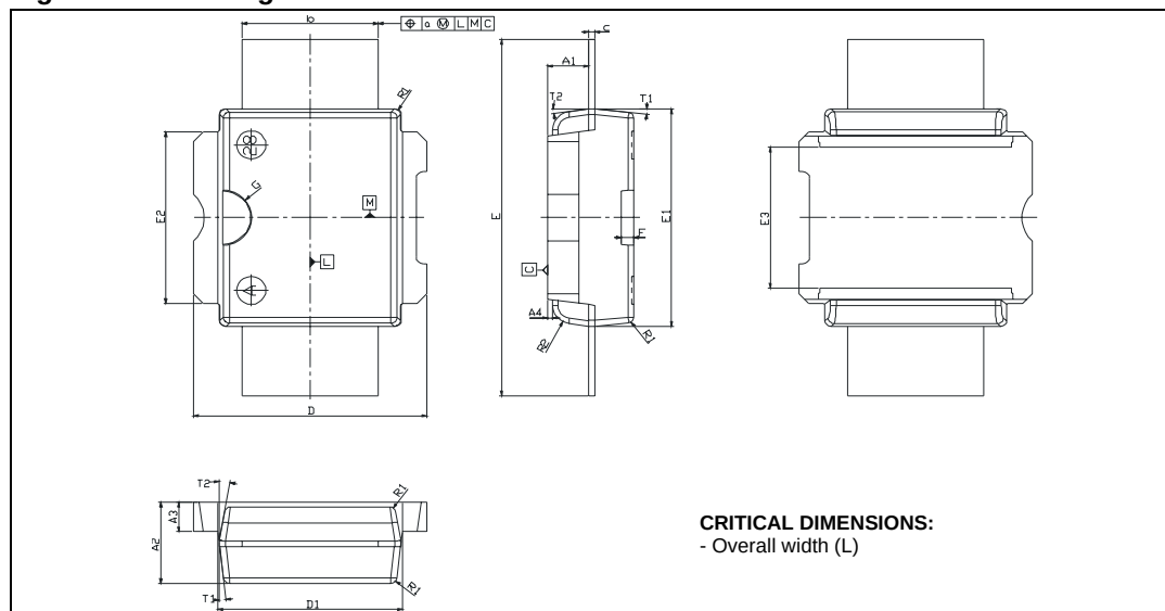
Figure 29. Package dimensions
