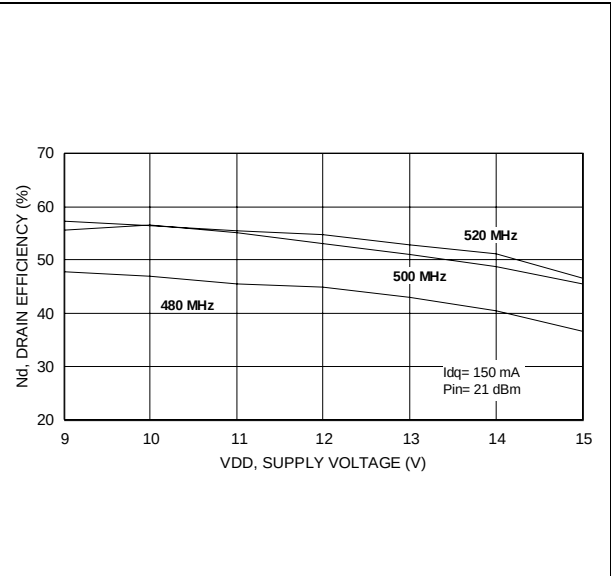
Figure 23. Drain efficiency vs. supply voltage
