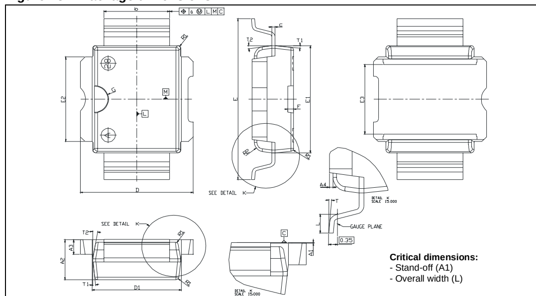
Figure 28. Package dimensions
