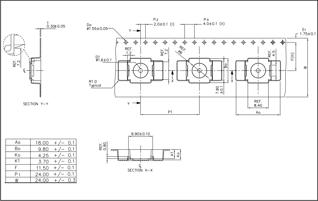
Figure 31. Reel information
