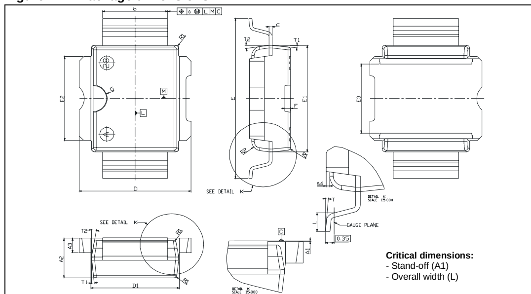
Figure 27. Package dimensions
