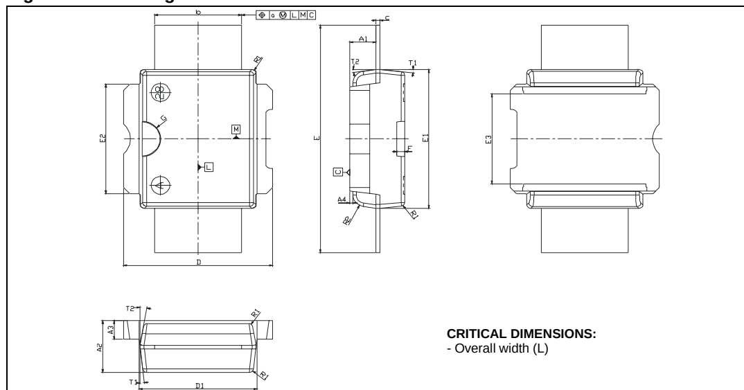
Figure 28. Package dimensions
