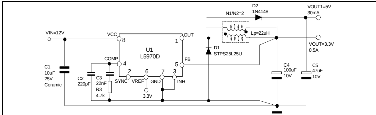
Figure 17. Buck-Boost regulator
