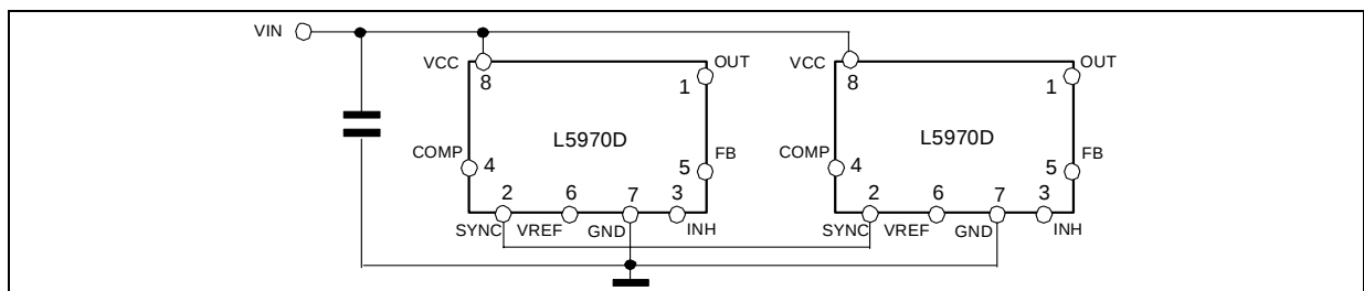
Figure 19. Synchronization example
