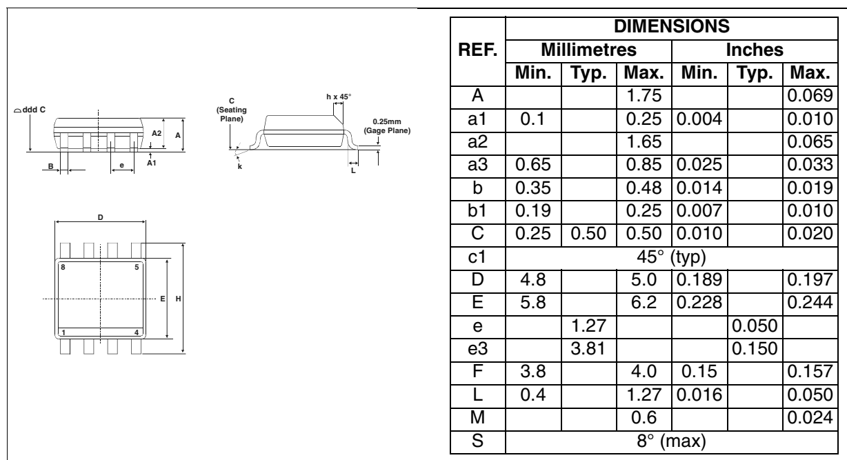
Figure 10: SO-8 Package Mechanical Data
