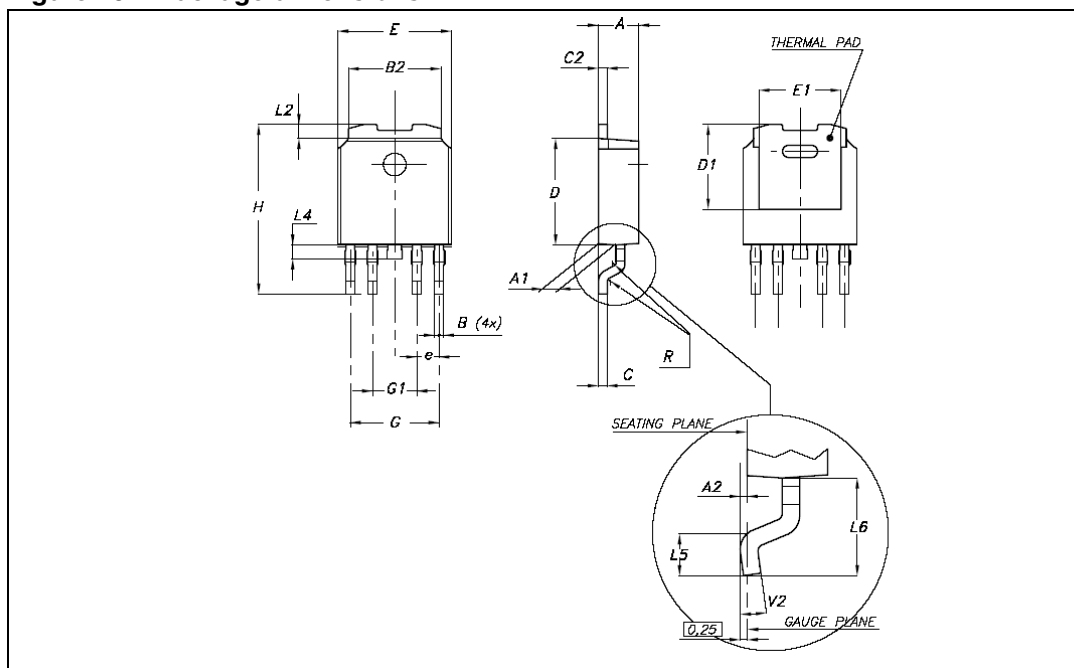
Figure 10. Package dimensions
