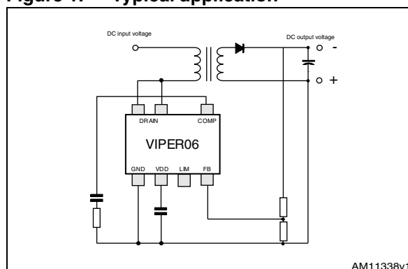
Figure 1. Typical application
