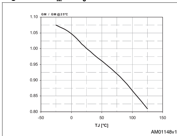
Figure 8. G_M vs. T_J
