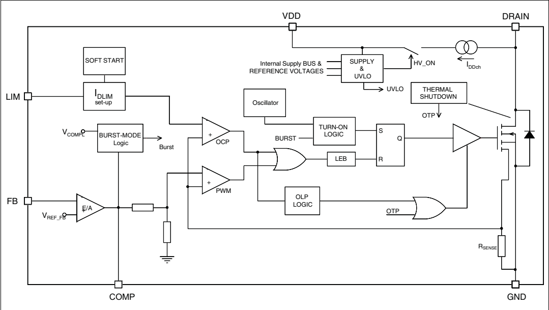
Figure 2. Block diagram
