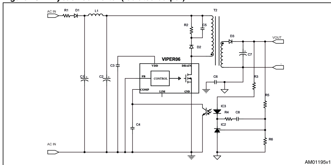
Figure 18. Flyback converter (isolated output)
