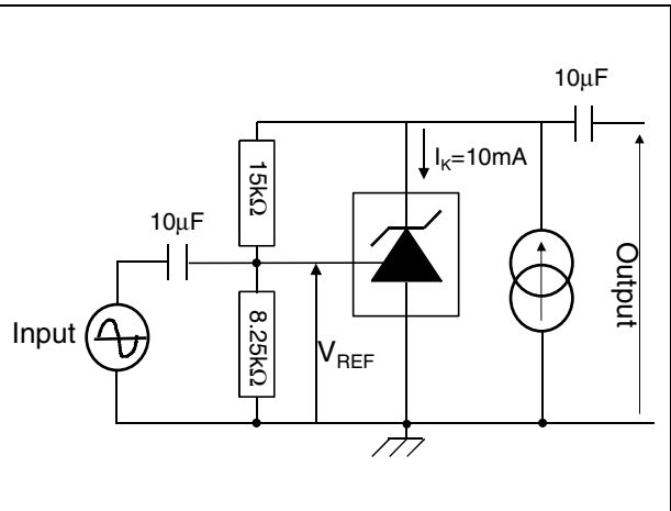
Figure 7. Test circuit for phase margin and voltage gain
