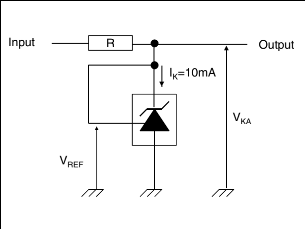
Figure 4. Test circuit V_{KA} = V_{REF}
