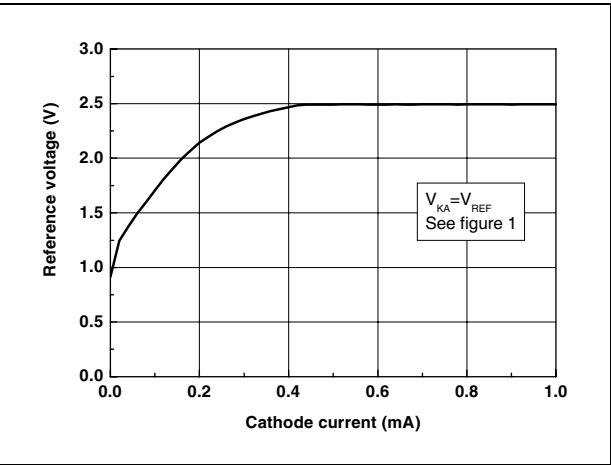
Figure 11. Reference voltage vs. cathode current ( I_K = 0 to 1 mA)
