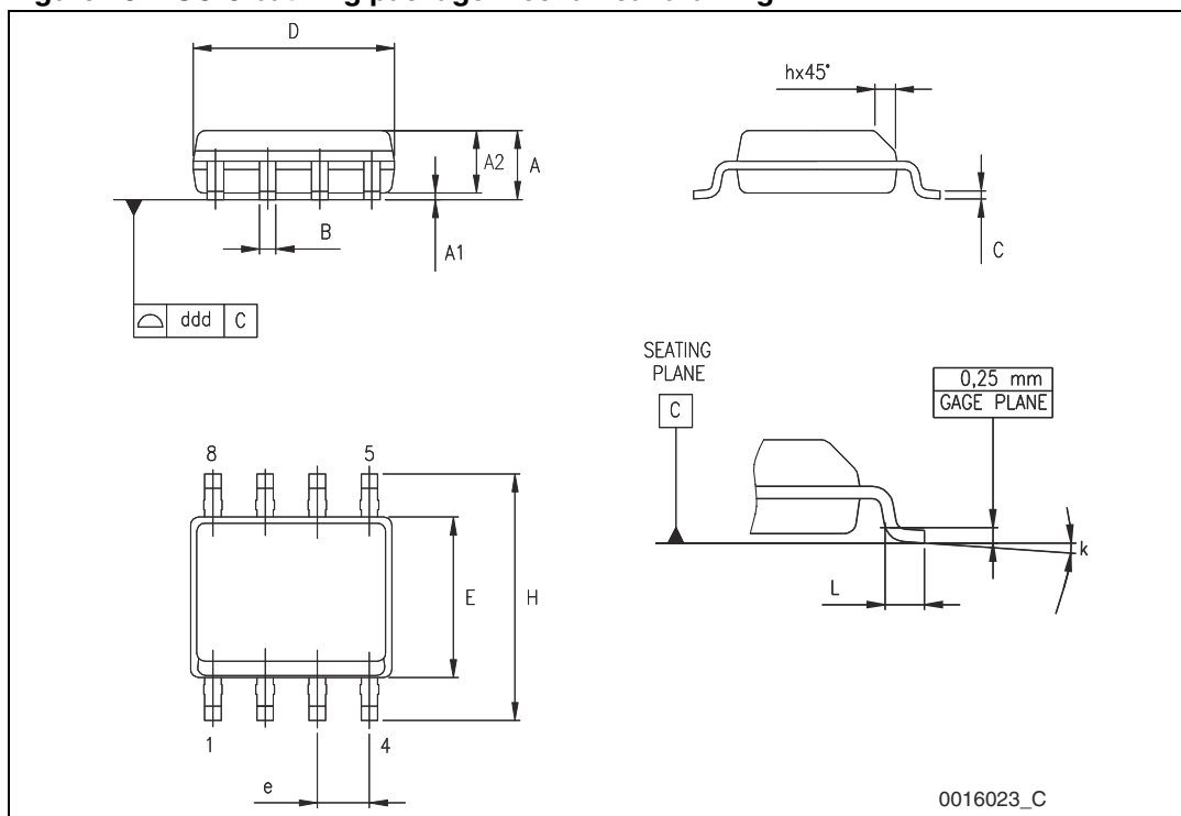
Figure 23. SO-8 batwing package mechanical drawing
