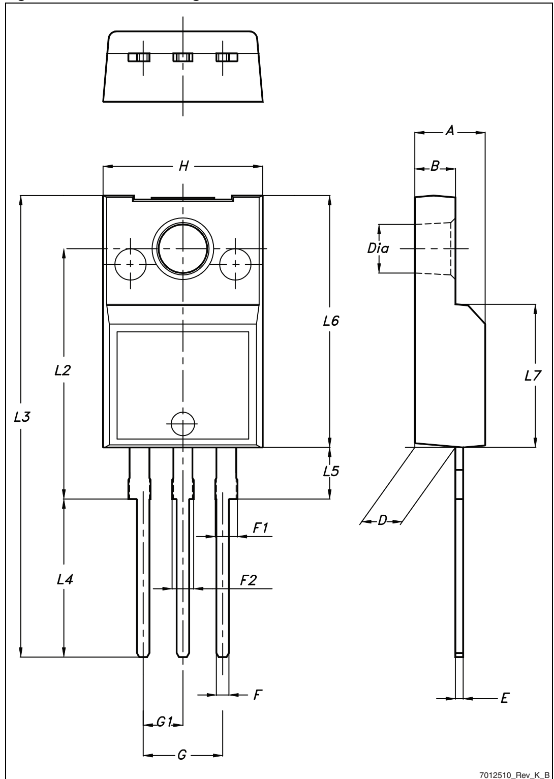
Figure 26. TO-220FP drawing
