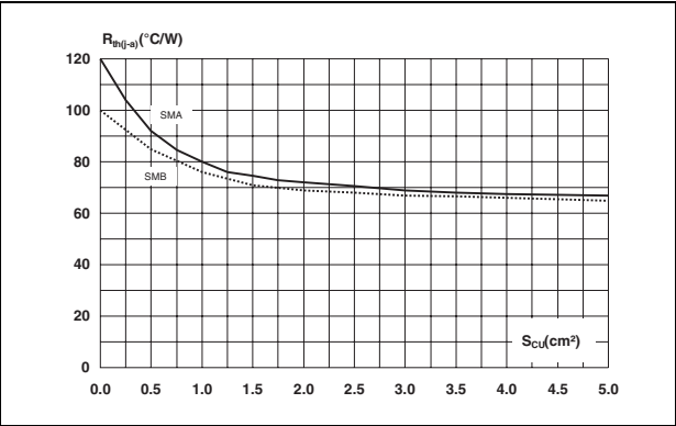
Figure 12. Thermal resistance, junction to ambient, versus copper surface under each lead - SMA/SMB (epoxy FR4, e_{Cu} = 35 \mu\text{m} )
