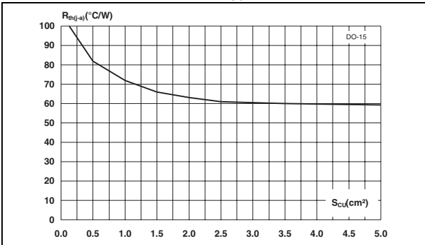
Figure 13. Thermal resistance, junction to ambient, versus copper surface under each lead DO-15 (epoxy FR4, e_{Cu} = 35 \mu\text{m} )
