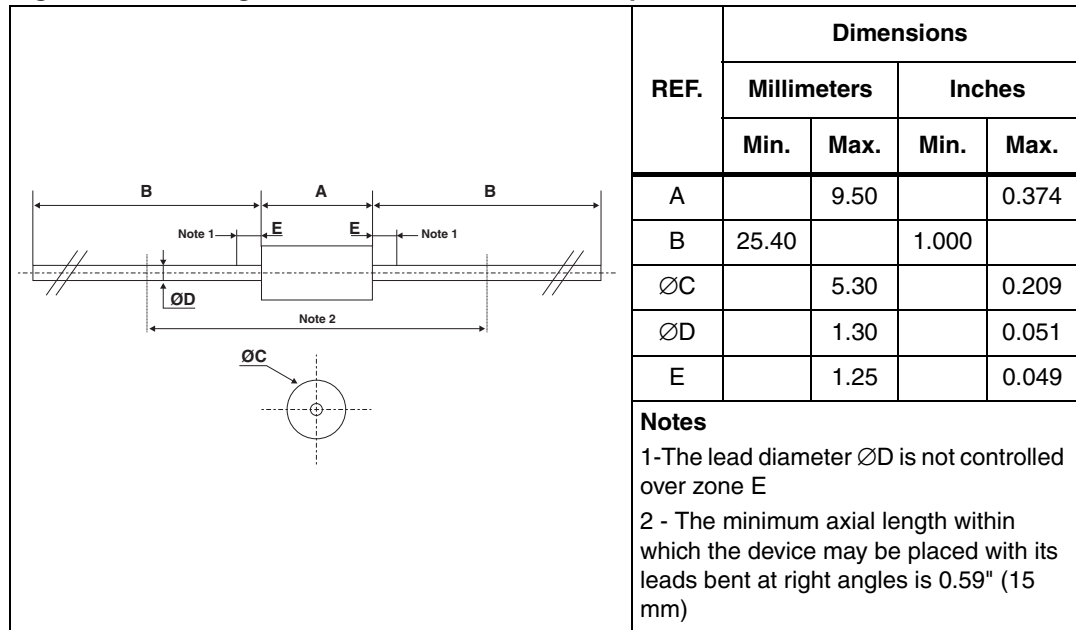
Figure 17. Package mechanical data DO-201AD plastic
