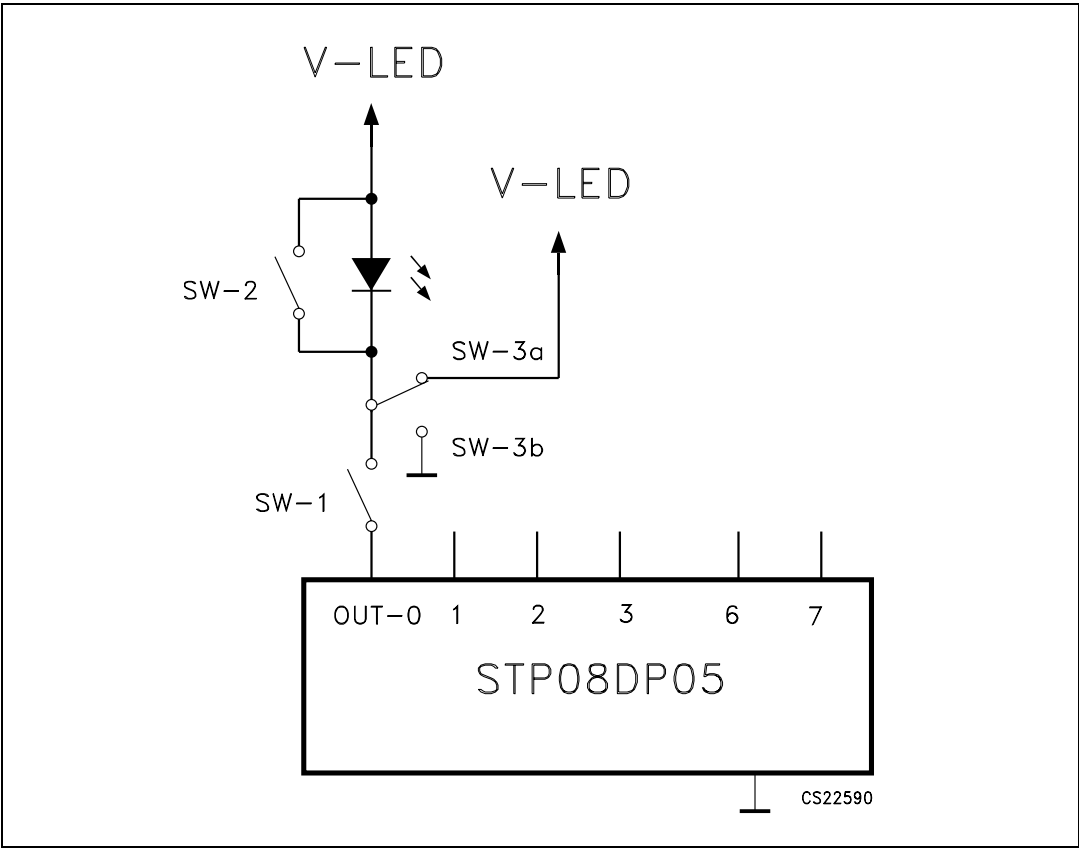
Figure 20. Detection circuit
