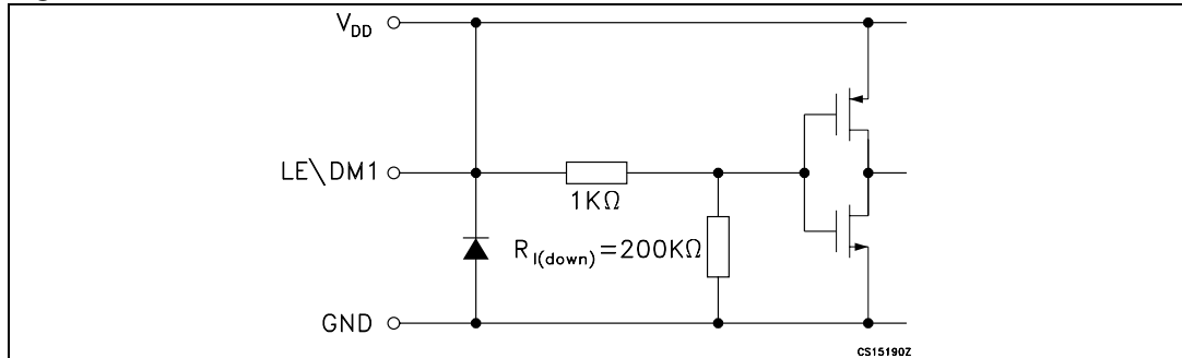
Figure 4. \text{LE}/\text{DM1} terminal
