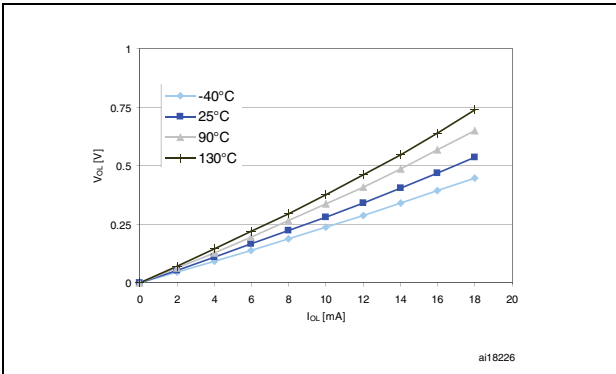
Figure 25. Typ. V_{OL} @ V_{DD} = 3.0 V (high sink ports)
