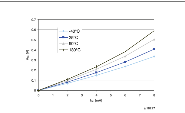
Figure 26. Typ. V_{OL} @ V_{DD} = 1.8 V (high sink ports)
