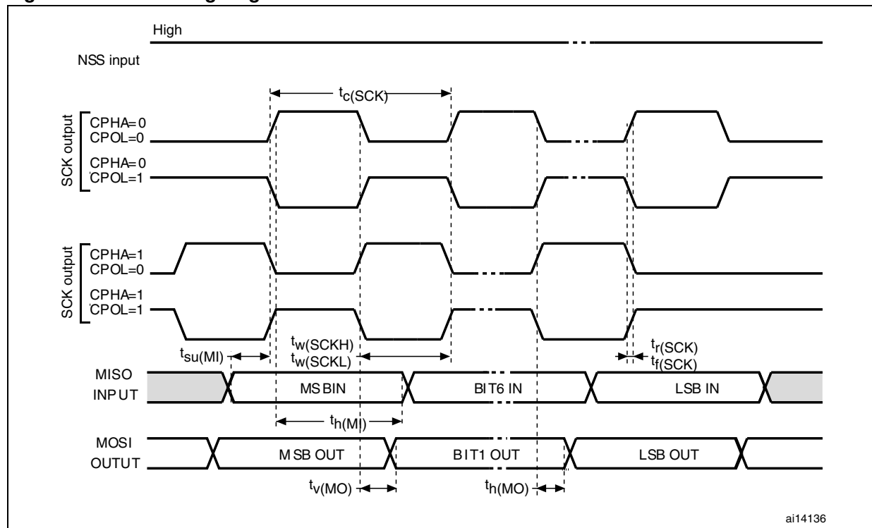
Figure 36. SPI1 timing diagram - master mode (1)
