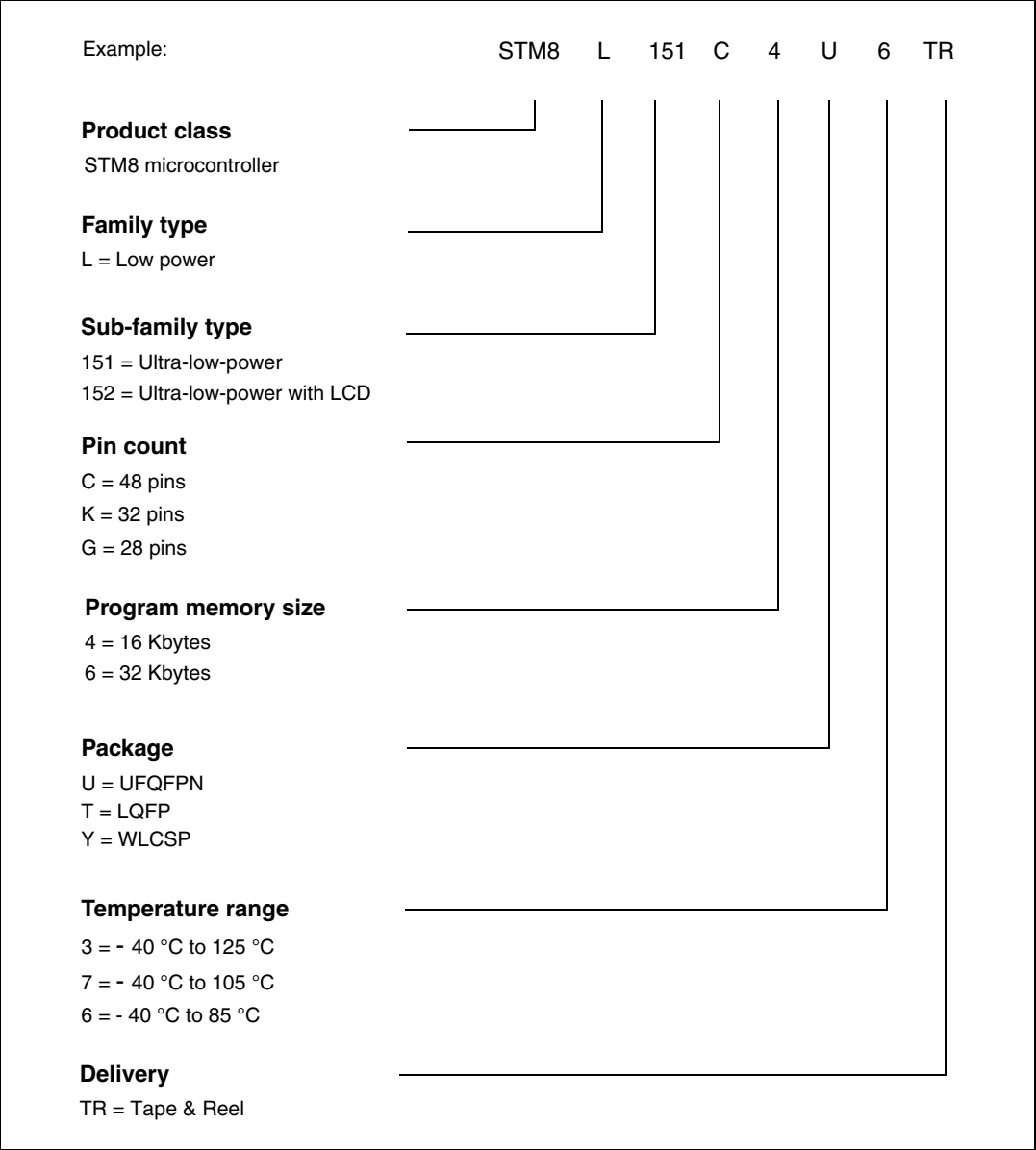
Figure 52. Medium density STM8L15x ordering information scheme
