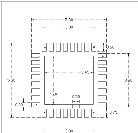
Figure 44. UFQFPN32 recommended footprint (1)(4)
