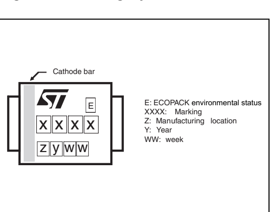
Figure 12. Marking layout
