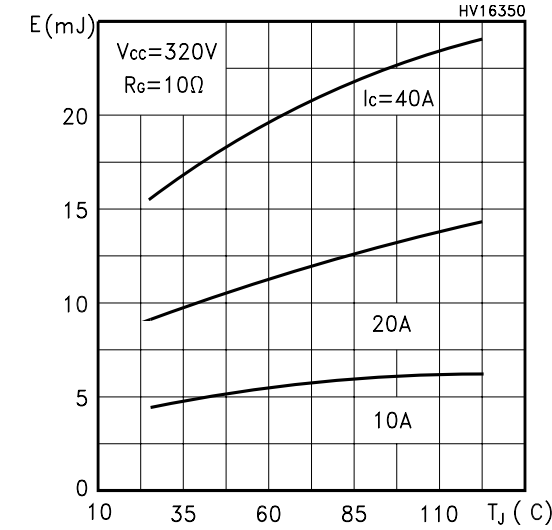
Off Losses vs Temperature
