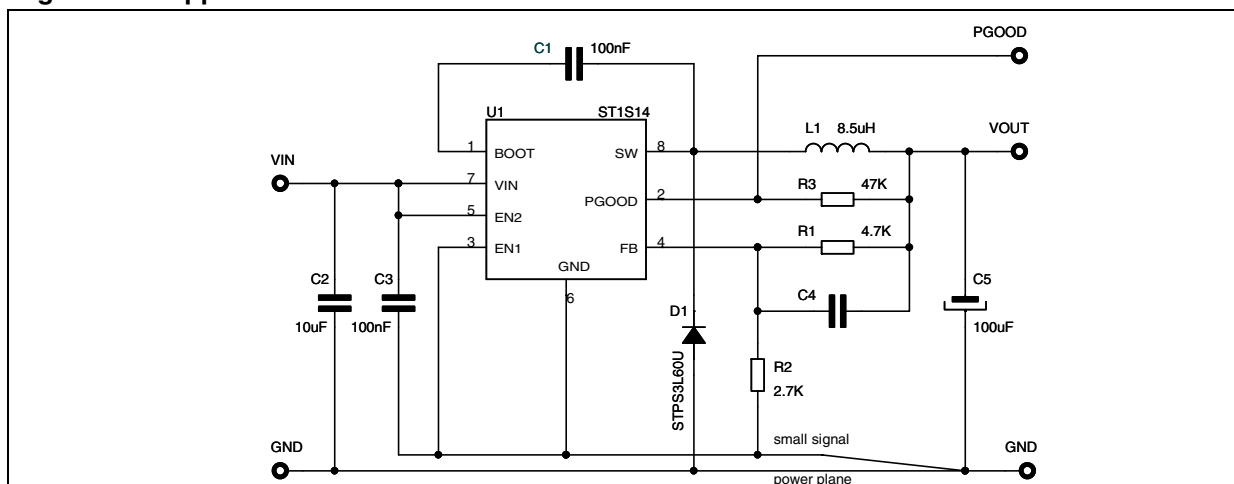
Figure 1. Application schematic
