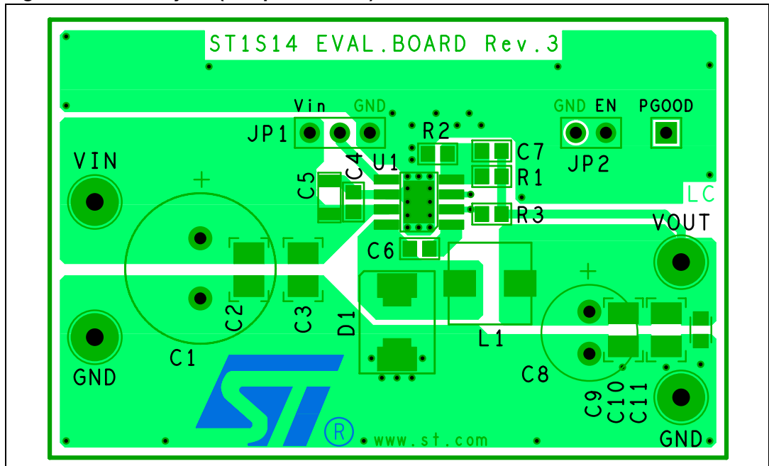
Figure 24. PCB layout (bottom side)
