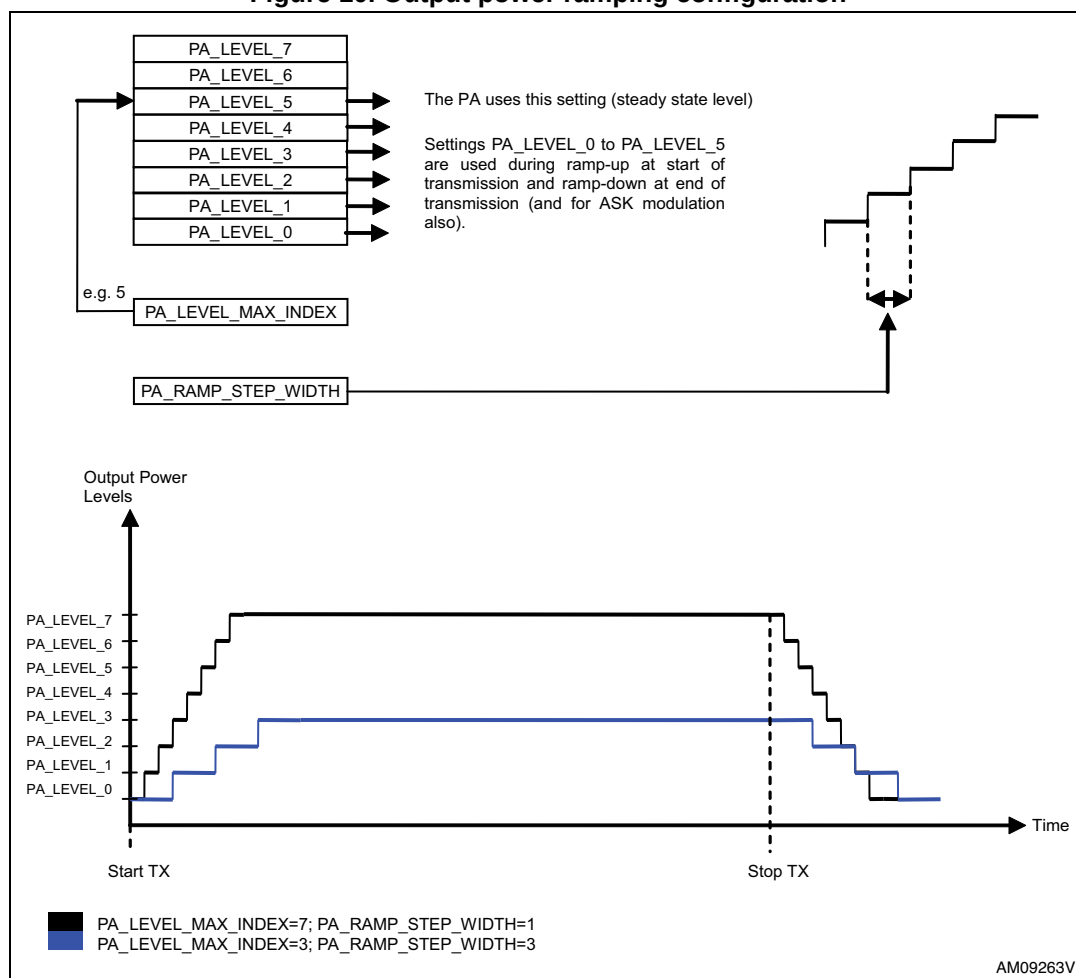
Figure 10. Output power ramping configuration
