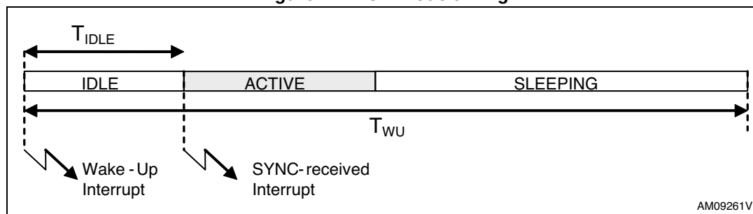
Figure 7. LDCR mode timing
