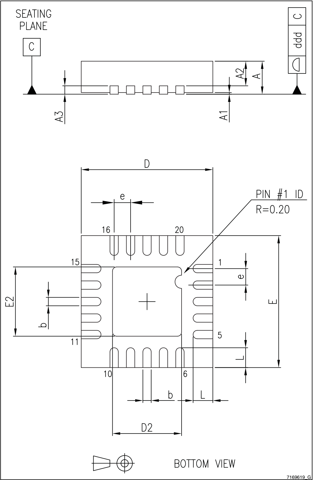
Figure 16. QFN20 (4 x 4 mm.) drawing dimension
