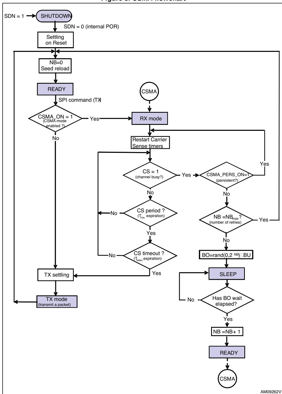
Figure 8. CSMA flowchart
