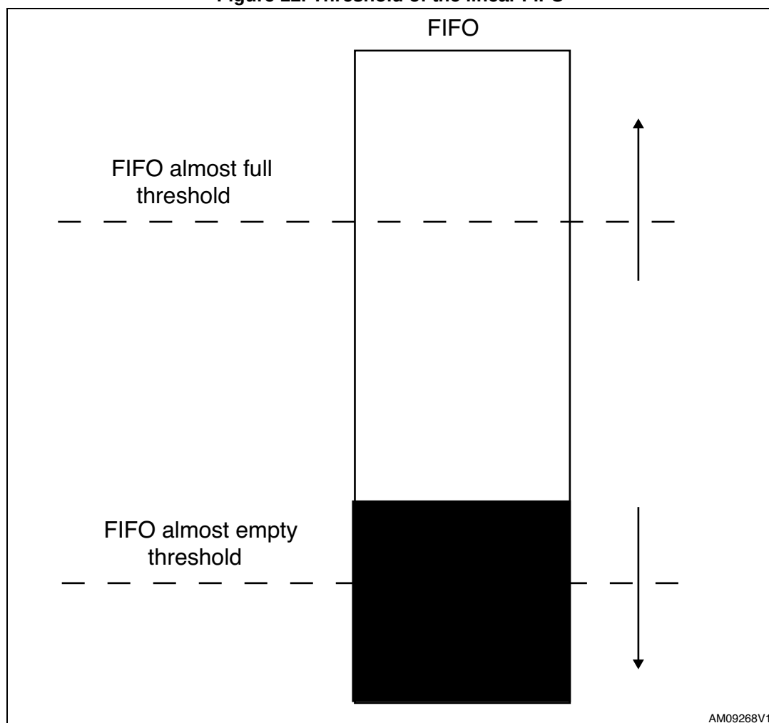
Figure 12. Threshold of the linear FIFO
