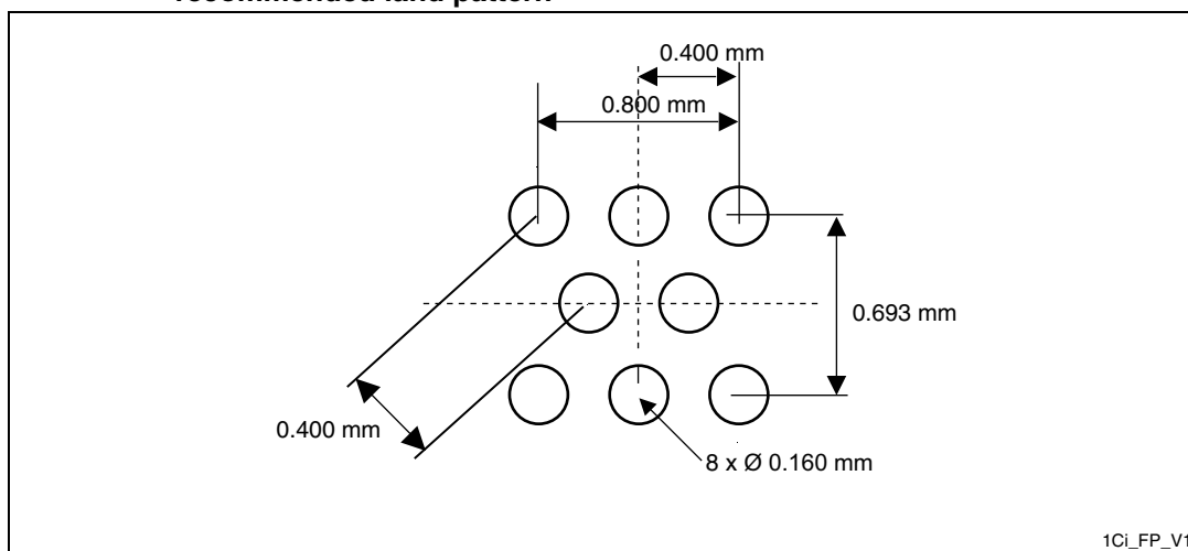
Figure 27. Thin WLCSP 8-bump wafer-length chip-scale package recommended land pattern
