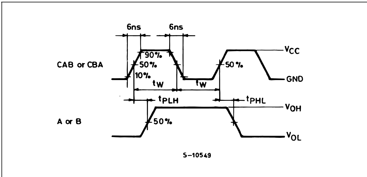
WAVEFORM 2 : PROPAGATION DELAY TIME, MINIMUM PULSE WIDTH (f=1MHz; 50% duty cycle)
