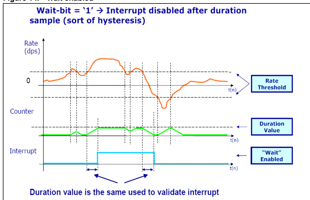
Figure 14. Wait enabled
