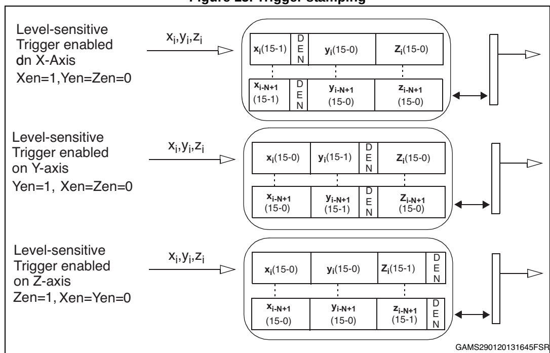
Figure 15. Trigger stamping
