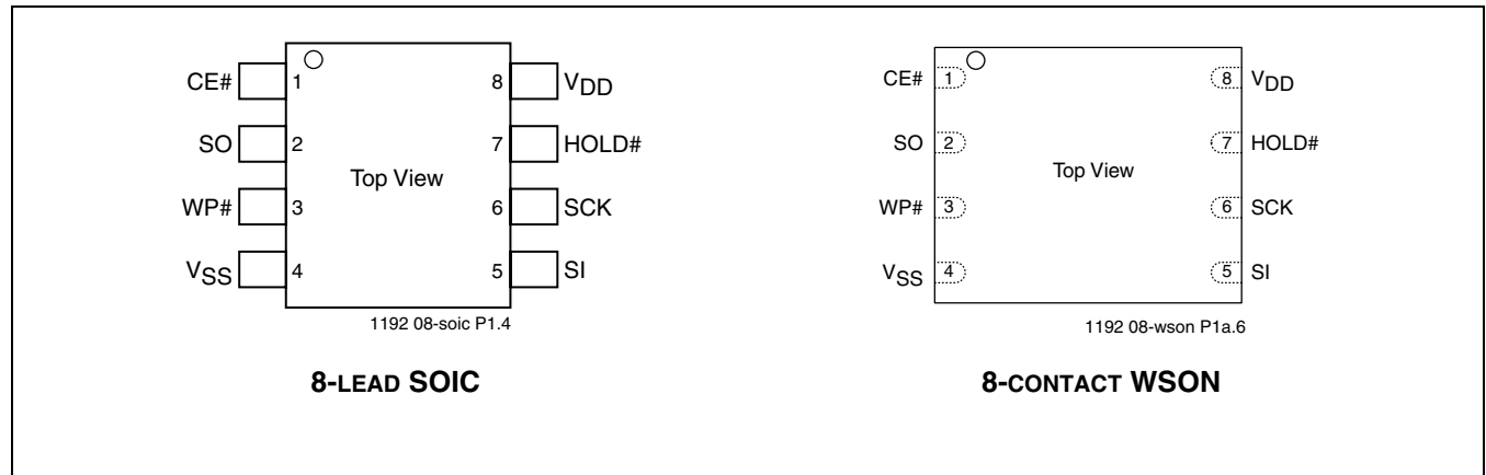
FIGURE 1: PIN ASSIGNMENTS
