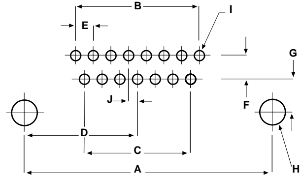
Printed Circuit Right Angle Mount (standard density)
