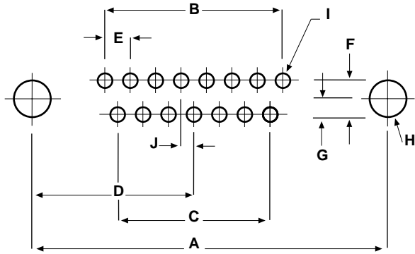
Printed Circuit Board Mount (standard density)
