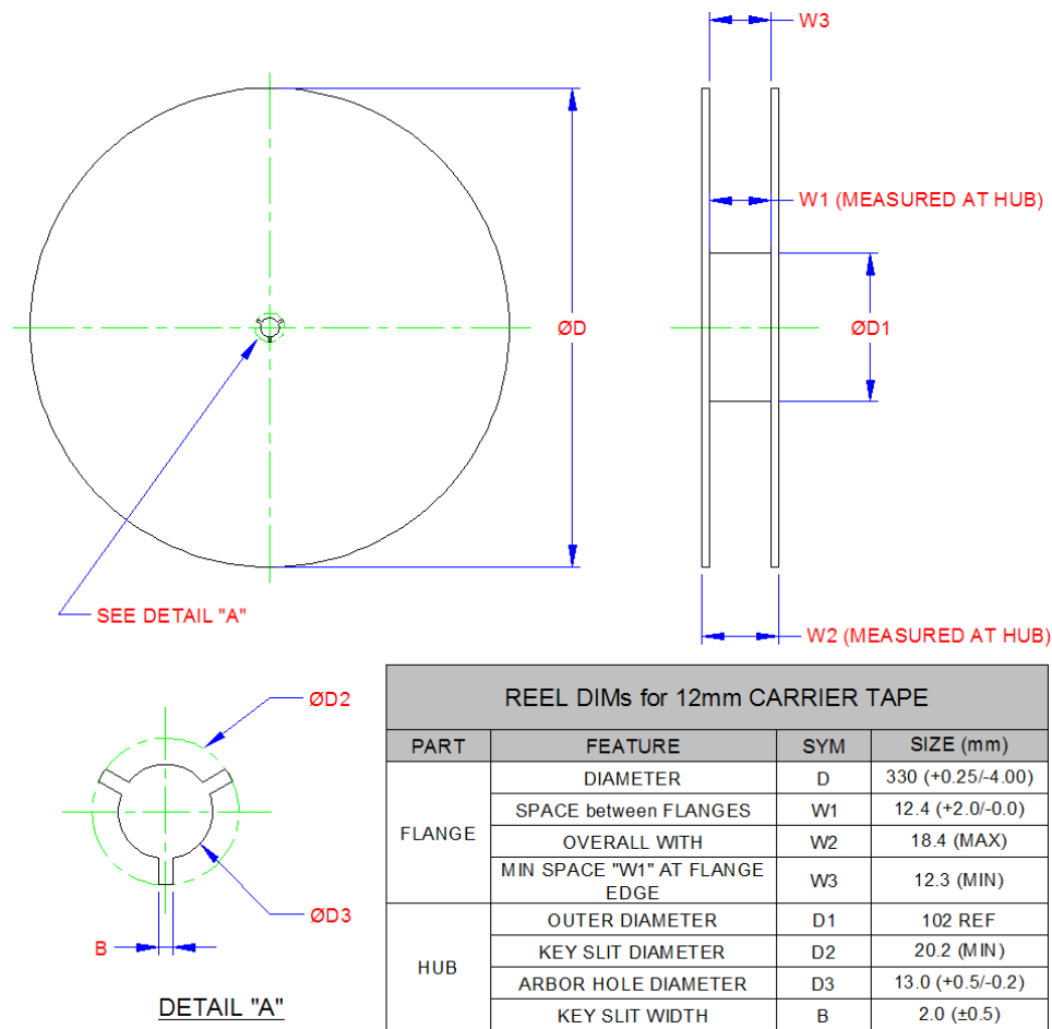
Figure 6.4 Reel Dimensions
