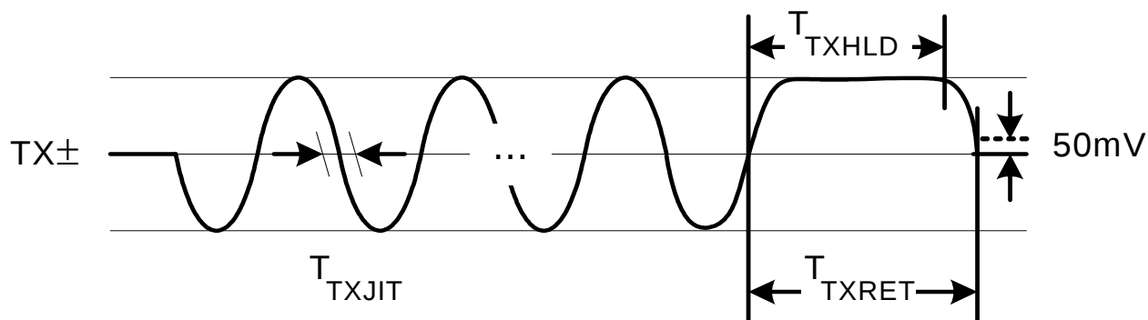
Figure 19. 10BASE-T Transmit
