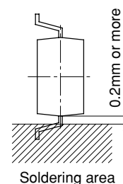
Soldering area
